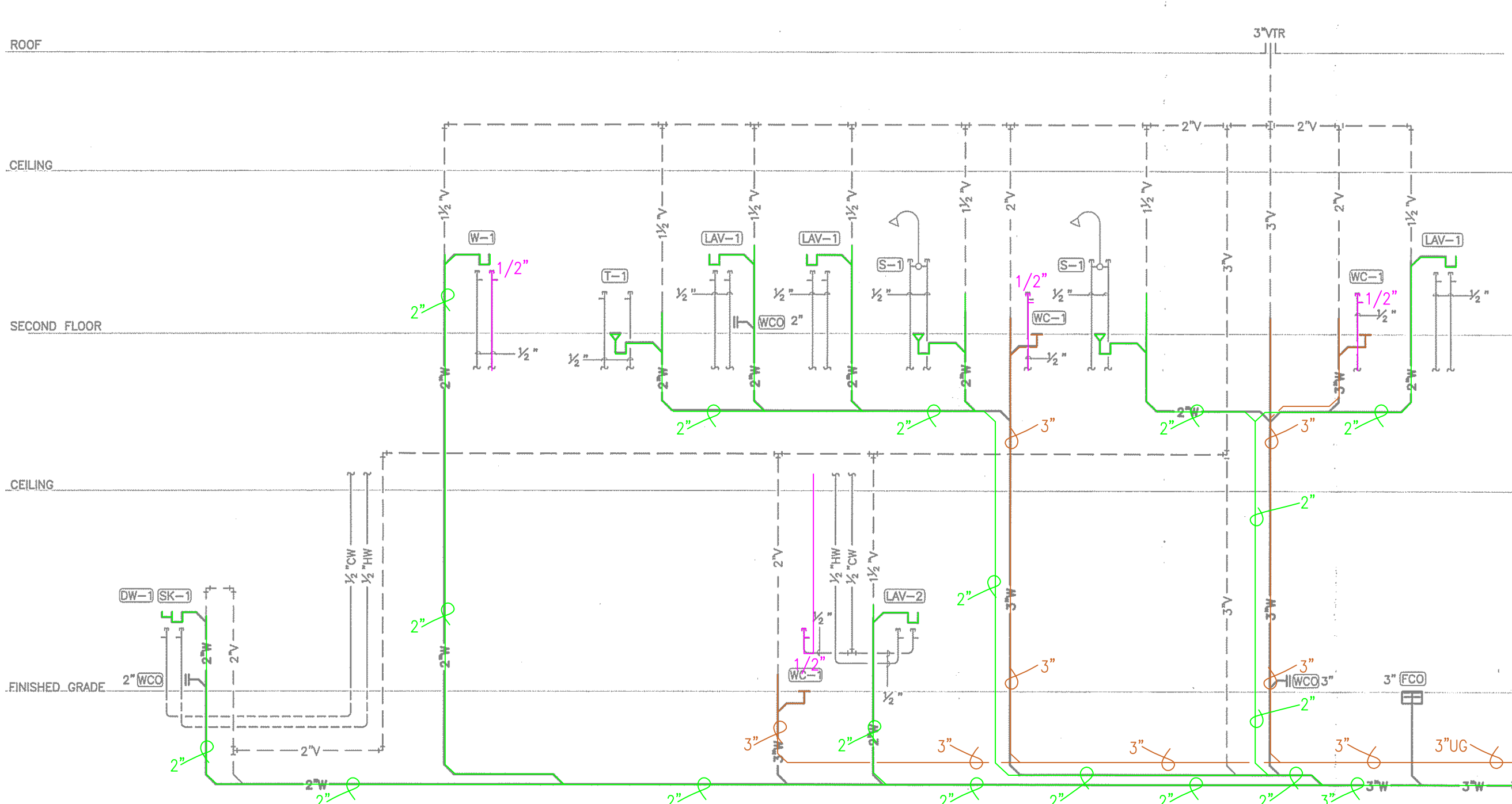
2 PLUMBING - RISER DIAGRAM UNIT B SCALE: NONE
