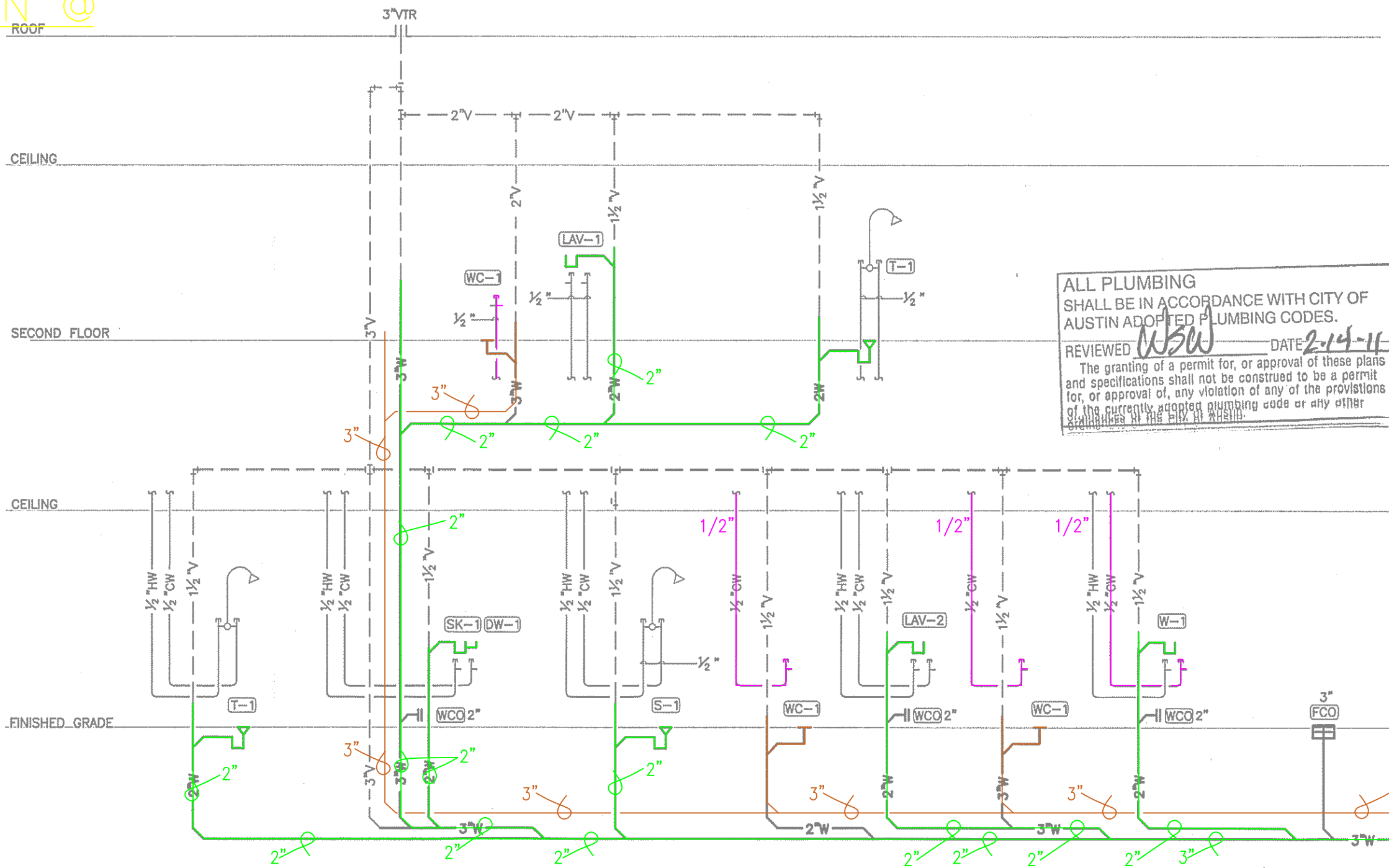
4 PLUMBING - RISER DIAGRAM UNIT D SCALE: NONE
